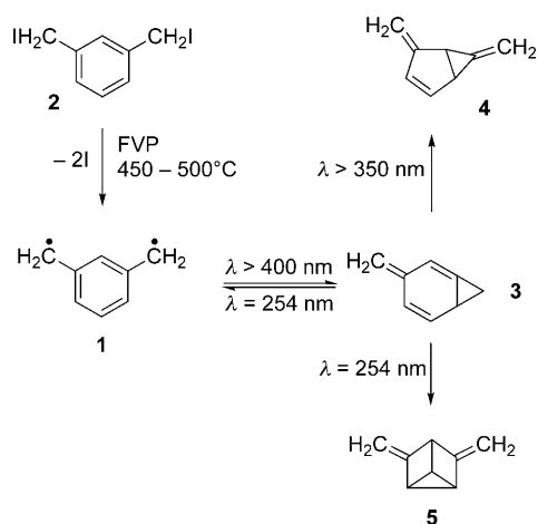
Scheme 1. Synthesis and photochemistry of m -xylylene 1 .
