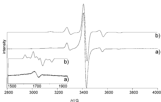
Figure 3. a) EPR spectrum obtained after irradiation of matrix isolated 7 with 308 nm. b) Simulated quartet EPR spectrum using |D/hc| = 0.0128 \text{ cm}^{-1} , |E/hc| = 0 \text{ cm}^{-1} , g = 2.0023 , \mu = 9.60067 \text{ GHz} . Inset: half-field signal.
