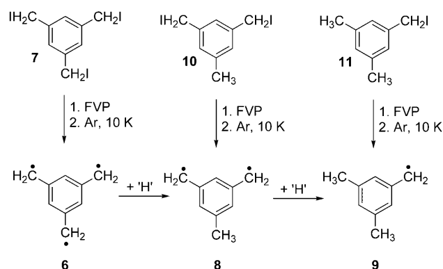
Scheme 2. Synthesis of 1,3,5-trimethylenebenzene 6 and by-products through flash vacuum pyrolysis.
