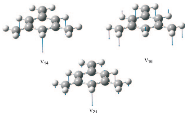
Figure 2. A_2'' symmetrical out of plane vibrations of 6 .
