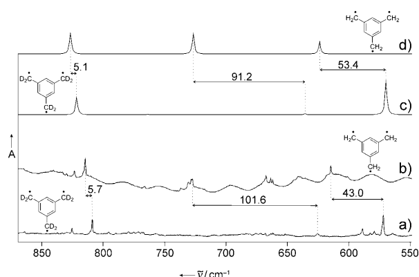
Figure 1. IR spectra obtained after FVP at 480 °C and subsequent trapping of the products in argon at 10 K. a) FVP of [D_6]-7 . b) FVP of 7 . c) IR spectrum of quartet [D_6]-6 calculated at the UB3LYP/6-311 + G(d,p) level of theory. d) IR spectrum of quartet 6 calculated at the UB3LYP/6-311 + G(d,p) level of theory.
